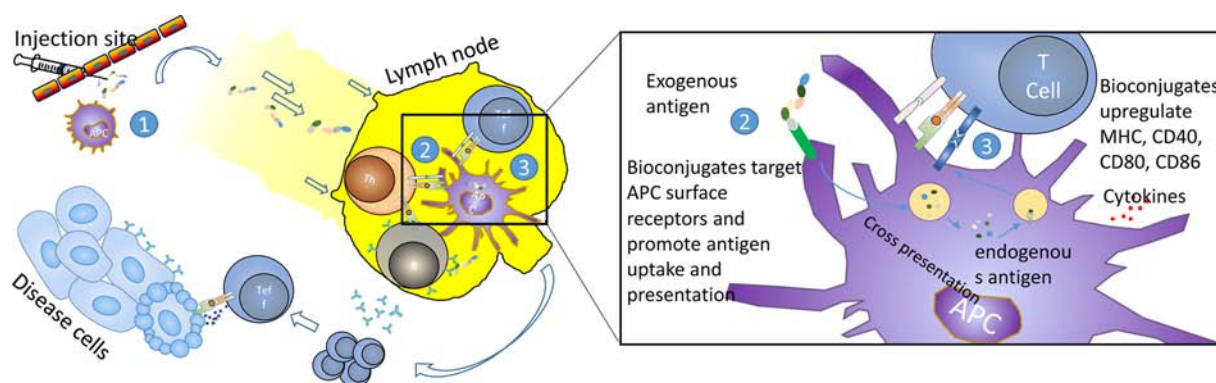
Figure 1. Mechanisms by which bioconjugates enhance the activation of immune system through vaccination. Activation of the immune response begins when vaccines are introduced to the body. Bioconjugates have been engineered to target vaccines to antigen-presenting cells (APCs) in the lymph node (1); to enhance the antigen uptake and presentation (2); and to activate APCs (3).
