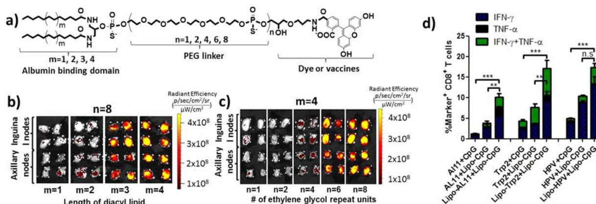
Figure 2. Targeting lymph nodes with “albumin-hitchhiking” vaccines. (a) Schematic of the design of albumin-binding amphiphiles. Antigen-amphiphiles contain a lipophilic albumin-binding diacyl lipid tail, PEG solubilizing linker, and a vaccine cargo (peptide or other antigen, or adjuvant compound). (b,c) Fluorophore-conjugated amphiphiles were injected s.c. in mice, and draining LNs were isolated and imaged 24 h post injection. Albumin-binding amphiphiles accumulated in LNs in a lipid (b, fixed PEG length 48 EG units) and PEG (c, fixed C18 diacyl lipid tails) molecular weight-dependent manner. (d) Following vaccination, “albumin-hitchhiking” vaccines (“Lipo” conjugates) elicited enhanced antigen-specific CD8 + T-cells responses compared to traditional peptide vaccines adjuvanted with the Toll-like receptor agonist CpG DNA. Shown are frequencies of antigen-specific cytokine-producing T-cells among all CD8 + T-cells in peripheral blood 7 days post boost. Reprinted by permission from Macmillan Publishers Ltd., ref 48, copyright 2014.
