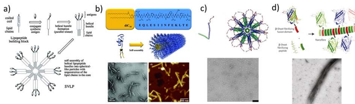
Figure 4. Monomeric peptides self-assemble into multivalent nanostructures. Lipid-conjugated peptide amphiphiles self-assemble into spherical (a) and cylindrical (b) micelles. Peptides with intrinsic self-assembling properties provide a platform for multivalent display of antigens in nanoparticle (c) and nanofiber (d) platforms. Reproduced with permission from (a) ref 90, Copyright 2011 John Wiley & Sons Ltd; (b) ref. 91, Copyright 2012 John Wiley & Sons Ltd; (c) ref. 92, Copyright 2009 The American Association of Immunologists, Inc.; and (d) ref. 95, Copyright 2014 Macmillan Publishers Ltd.
