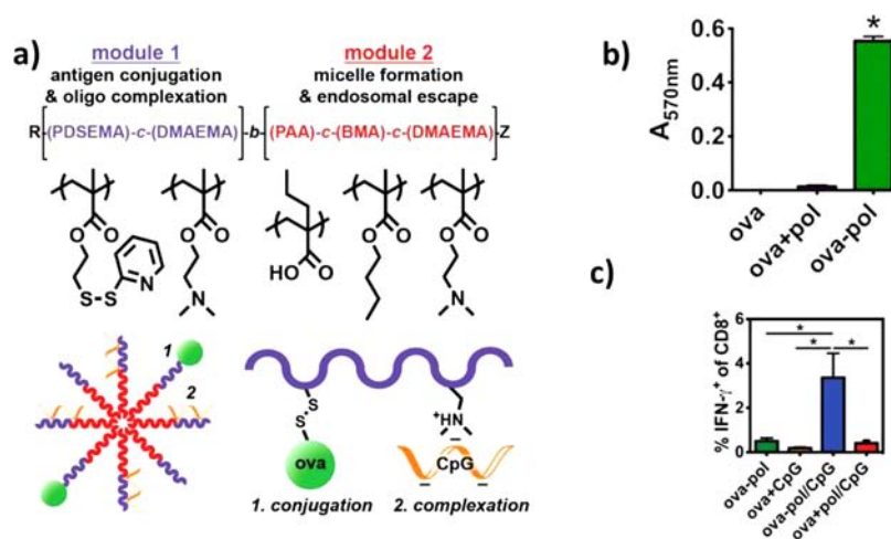
Figure 3. Synthesis and antigen conjugation of pH-responsive endosomolytic polymers for vaccine delivery. (a) Amphiphilic diblock copolymers were constructed with a hydrophilic block for antigen conjugation and a hydrophobic/endosomolytic block for promoting cytosolic antigen delivery. (b) Conjugation of ovalbumin (ova) antigen to the diblock polymeric carriers (pol) of panel (a) promoted MHC class I antigen presentation, as read out by production of LacZ (reported as an optical density at 570 nm) by a T-cell hybridoma reporter cell line incubated with dendritic cells loaded with the antigen. (c) Dual delivery of ova antigen and CpG adjuvant on the pH-responsive polymer conjugate enhanced cellular responses in vivo, as determined by measuring the frequency of IFN- \gamma -producing CD8 + T-cells following immunization. Reprinted with permission from ref 61, copyright 2013 American Chemical Society.
